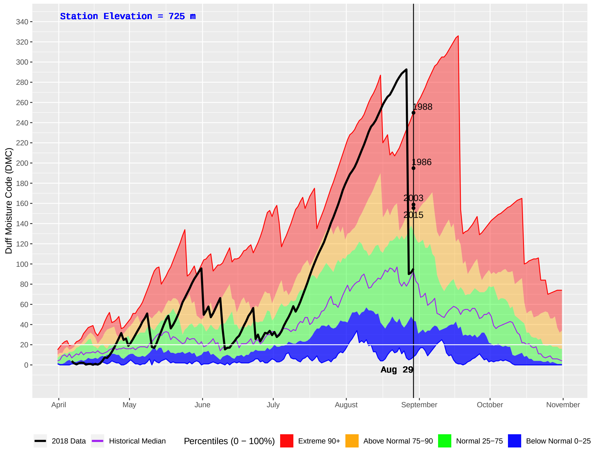
PENDOREILLE (402) : Historical (1986–2016) and Current (2018) Daily Duff Moisture Code (DMC)
