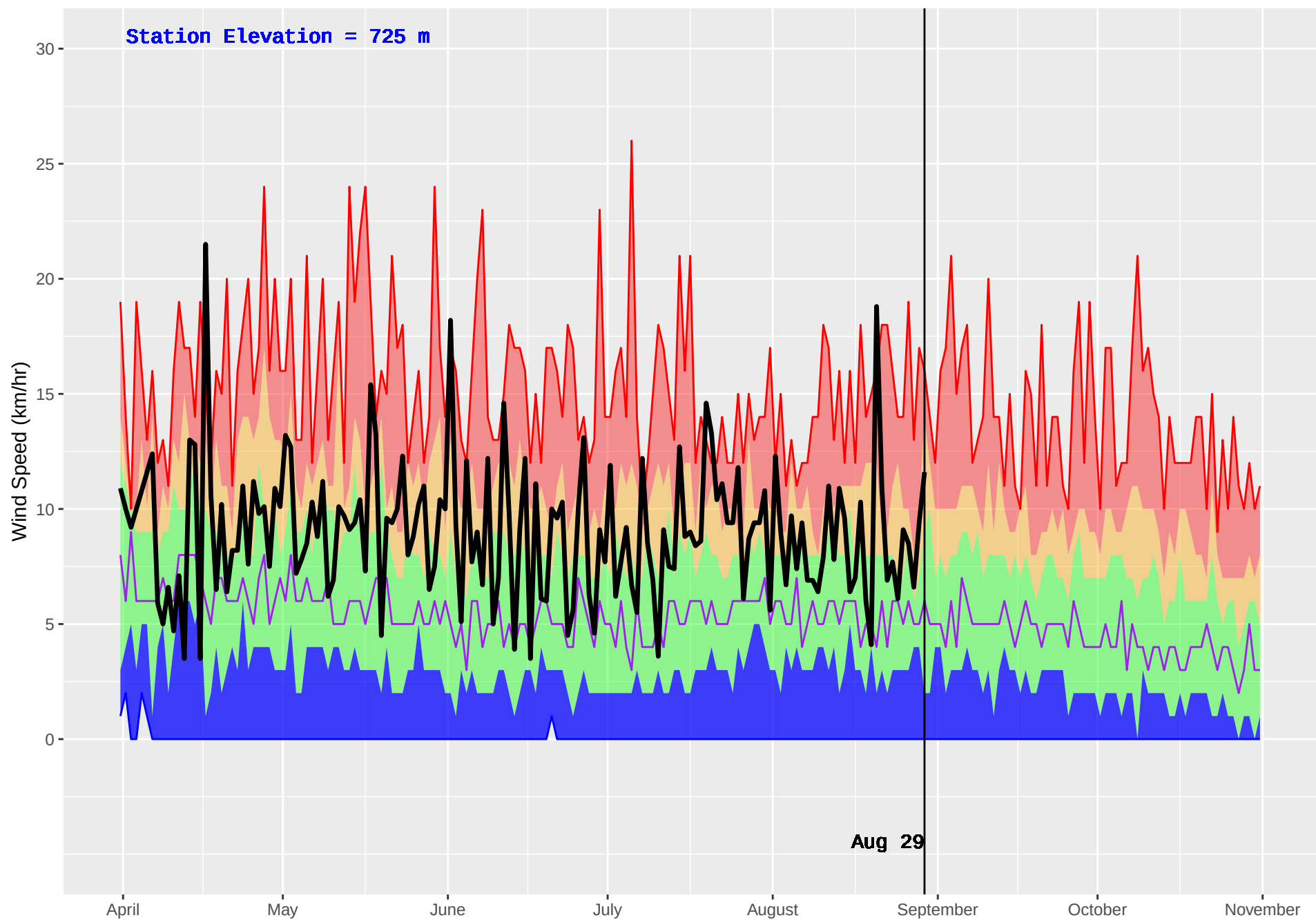
PENDOREILLE (402) : Historical (1986–2016) and Current (2018) Daily Wind Speed
